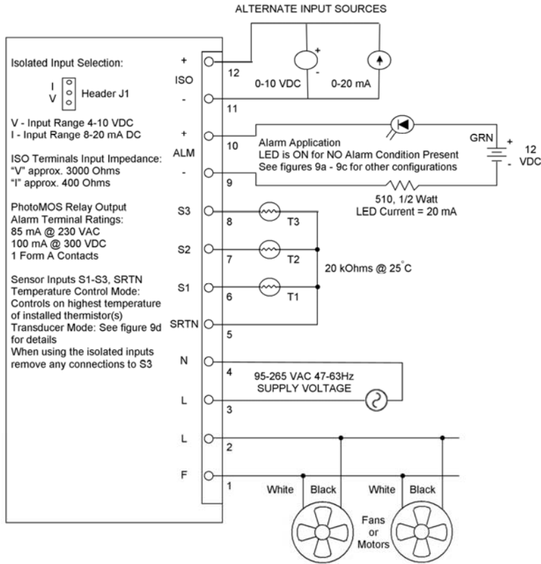
Figure 9: Wiring Diagram
